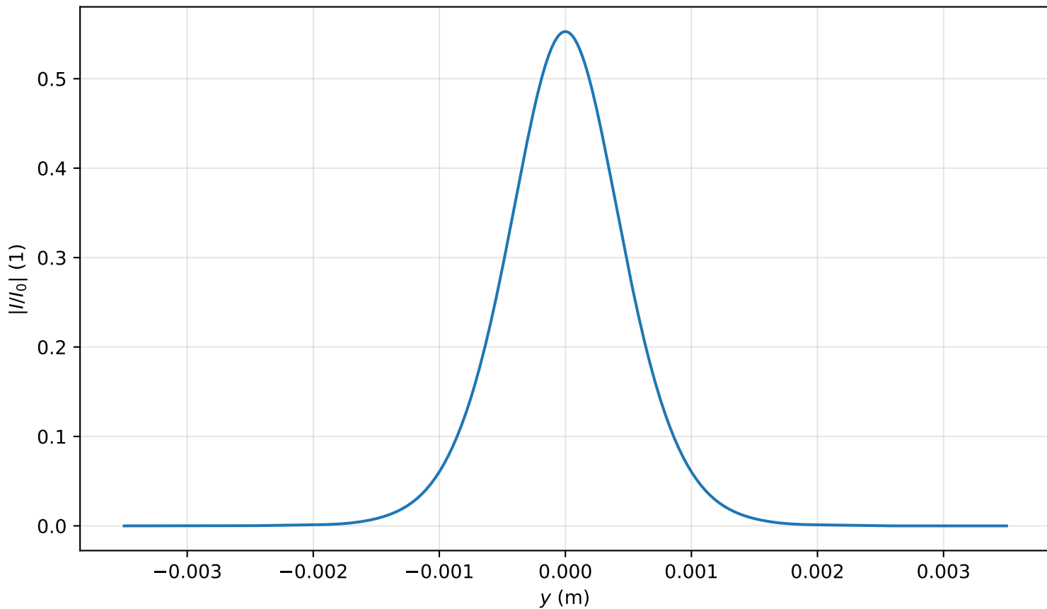
Intensity profile I(x=0, y, z=3.582)/I_0 , P_{in}=0.6P_{cr} , artificial time
